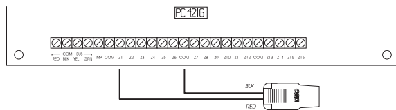
Figure 6, LED Assembly wiring
